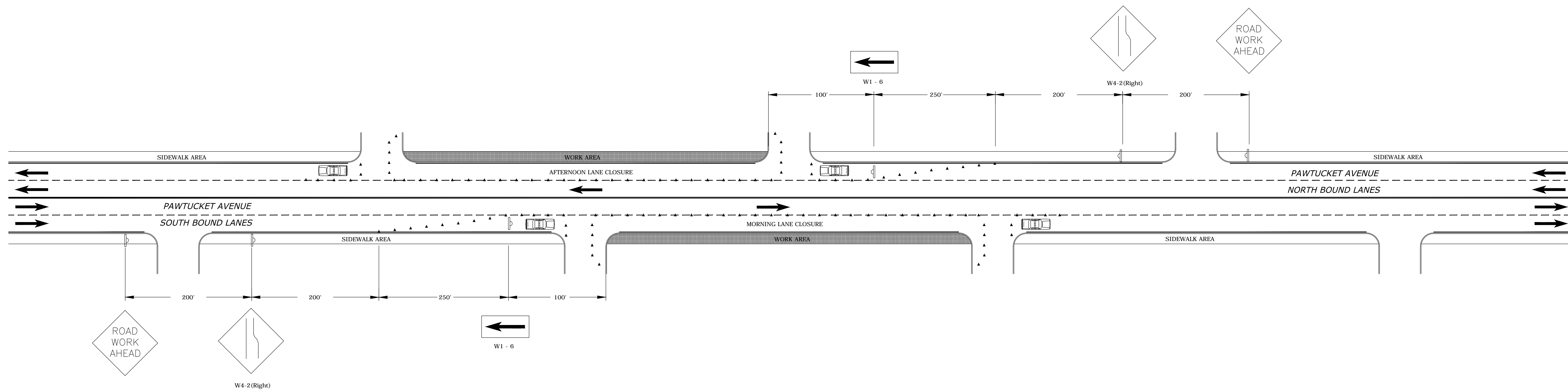
PAWTUCKET AVENUE ALTERNATING ONE LANE CLOSURE (TYP)
