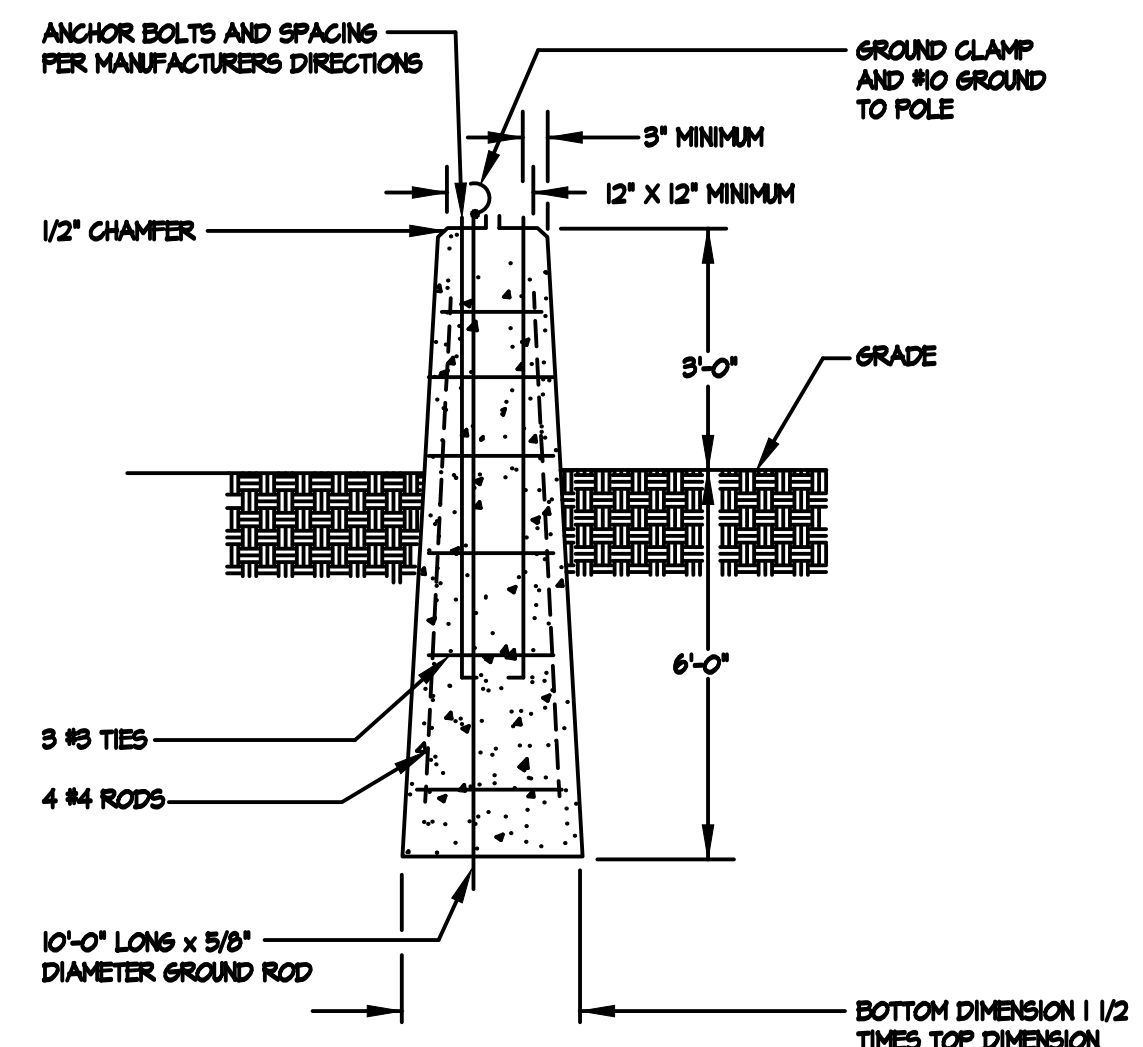
POLE BASE DETAIL NOT TO SCALE
